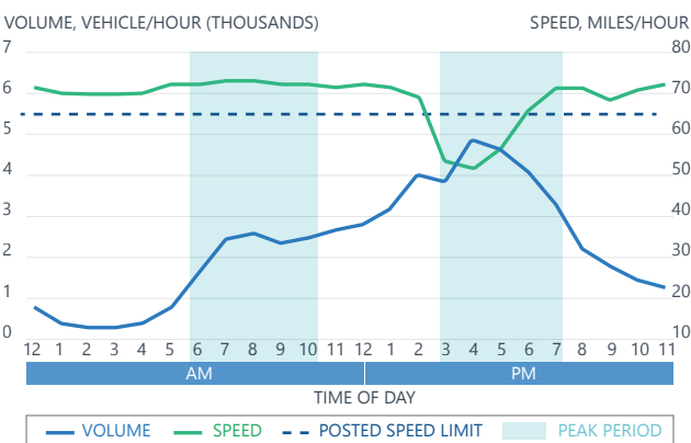
Figure 23. AET 8 Gantry Data, Westbound
