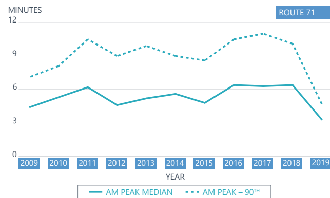
Figure 61. Route 71 Dedicated Bus Lane Run Times, AM Peak 2009–2019
