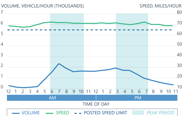
Figure 21. AET 4 Gantry Data, Westbound
